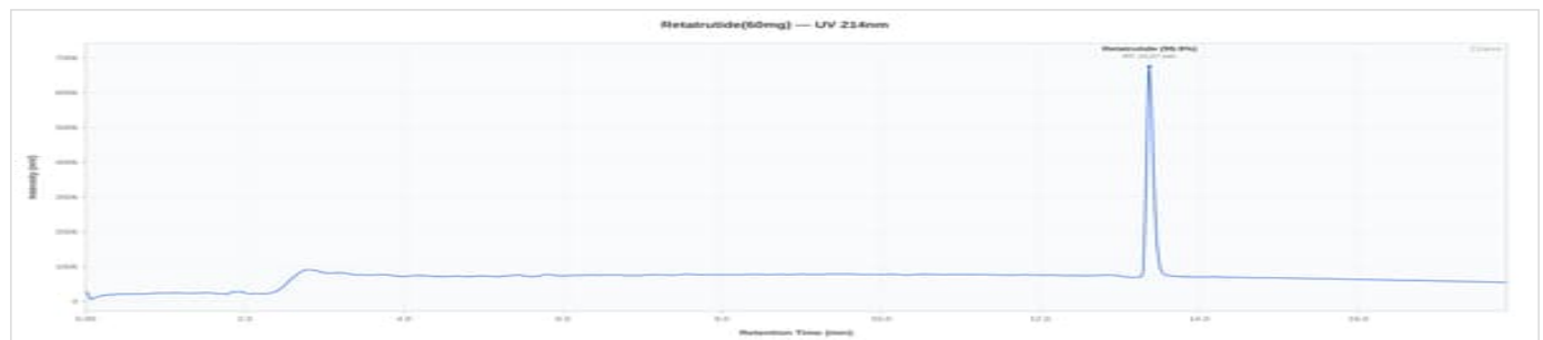
GLP-3 R 60mg - PL-RT60-01: UV Chromatogram
